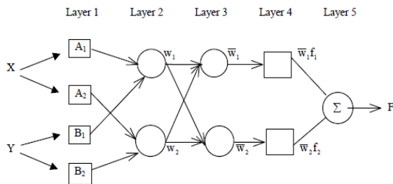
Figure4.Schematic diagram of an ANFIS structure with two inputs.
