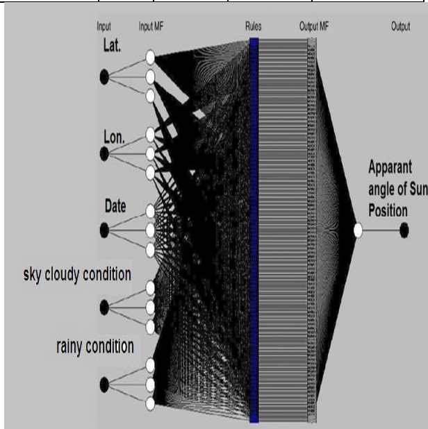
Figure.6. Structure of the ANFIS designed in this study to predict apparant angle of sun position
