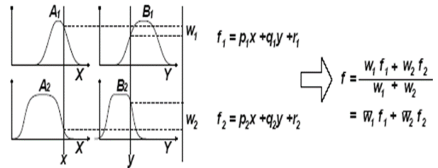
Figure5. Weighted summation of f_1 and f_2 in ANFIS to gain f as output.
