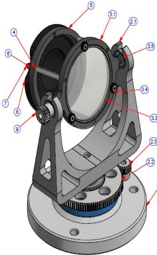
Figure3.3D view of Mechanical structure of the designed sun tracker lens (for description of the parts see Table1).
